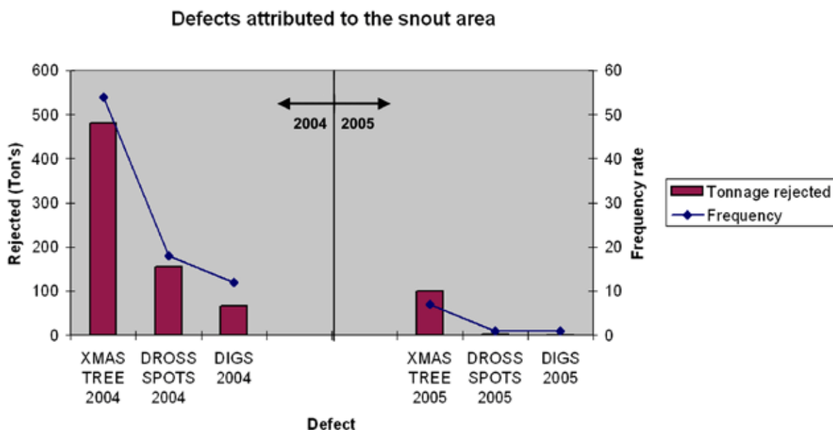
Graph illustrating the difference in strip defects at the customer in the first 5 months of 2004, compared to the same period in 2005. Ref.: “Cleanliness Enhancement of the Bath Surface within a CGL Snout”, C. Phillips, N. Staples & M. Bright, 97th Annual Meeting, Galvanizer’s Association, October 2005; recipient of 2005 Outstanding Author Award, Galvanizer’s Association
